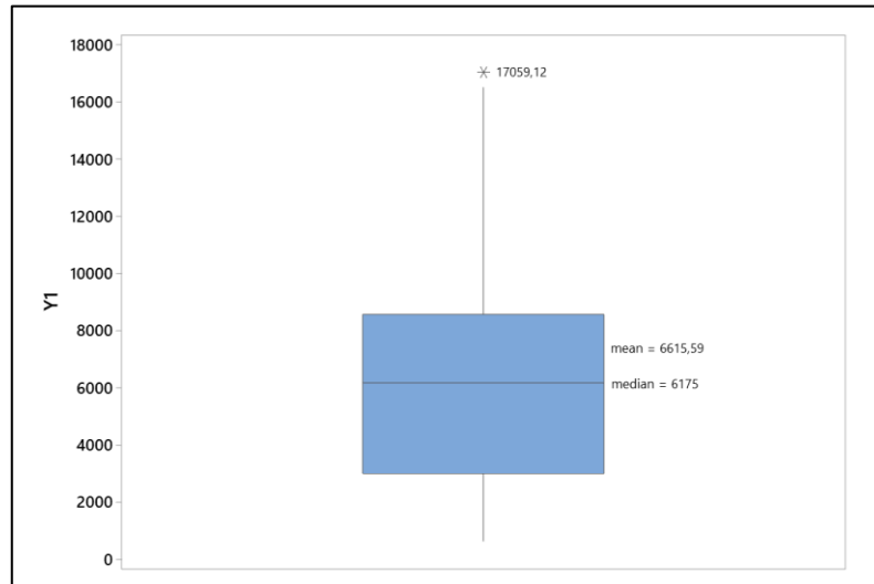
Gambar 2. Boxplot Harga Mobil
